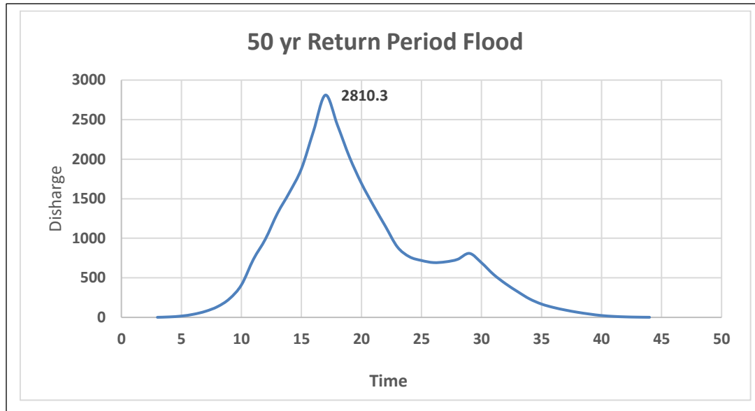
Fig.12: Design Flood Hydrograph for 50yr Return Period
