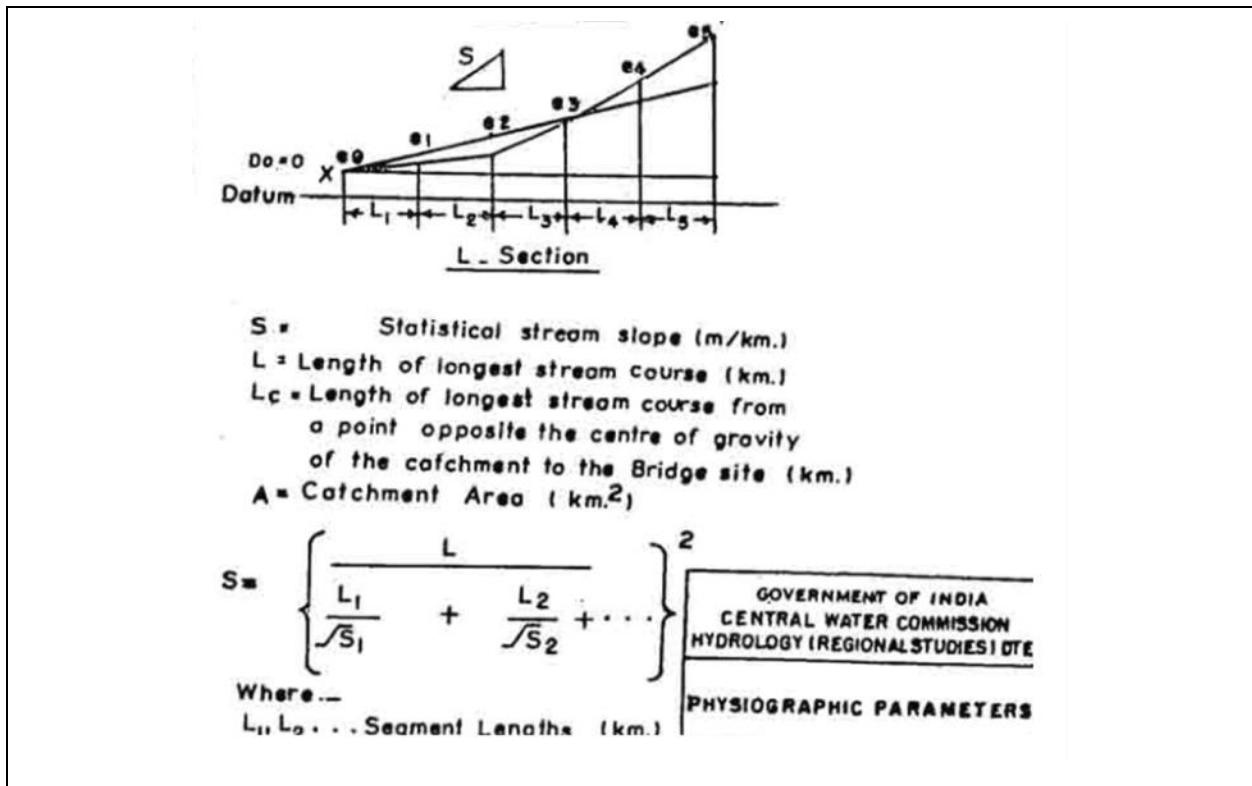
Fig.-5 Slope and other physiographic parameter calculation
