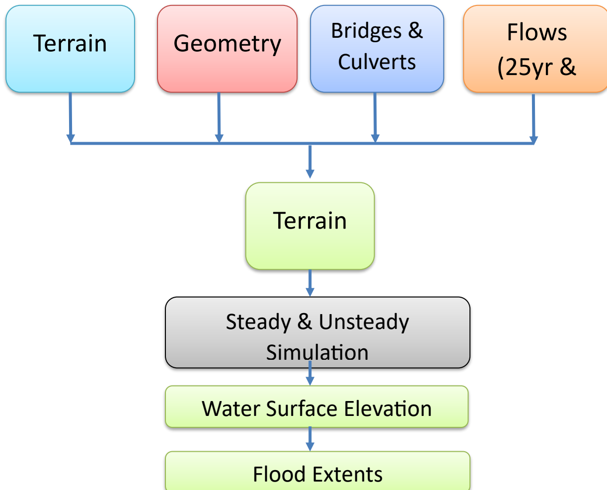
Fig. 18: Flow chart for modelling steps
