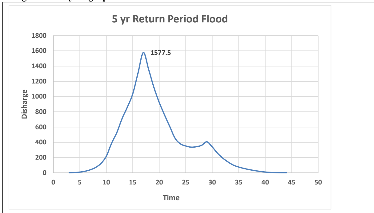
Fig.14: Design Flood Hydrograph for 5yr Return Period
