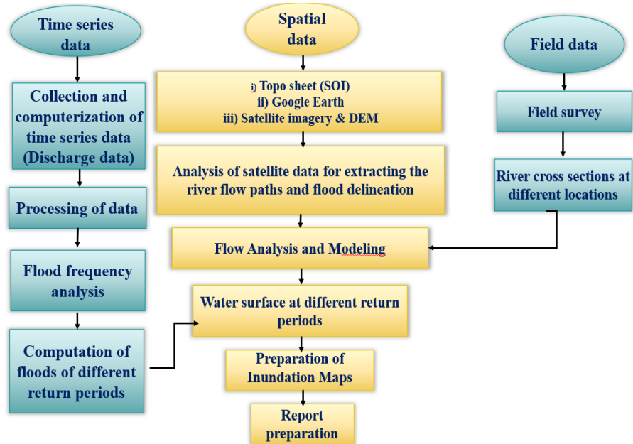
Fig.2 Flowchart of methodology of Flood Plain Zoning
