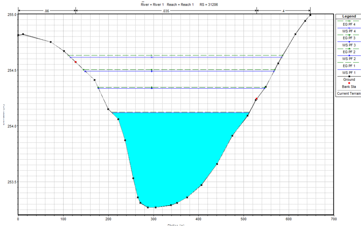
Fig. 20 Transverse cross-section at Roorkee showing N values.
