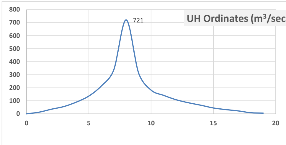
Fig.- 10: Synthetic Unit Hydrograph for Solani River
