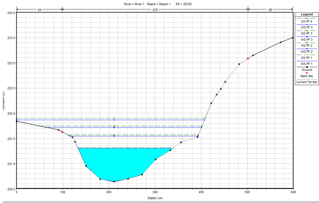
Fig. 20 Transverse cross-section at Roorkee showing N values.
