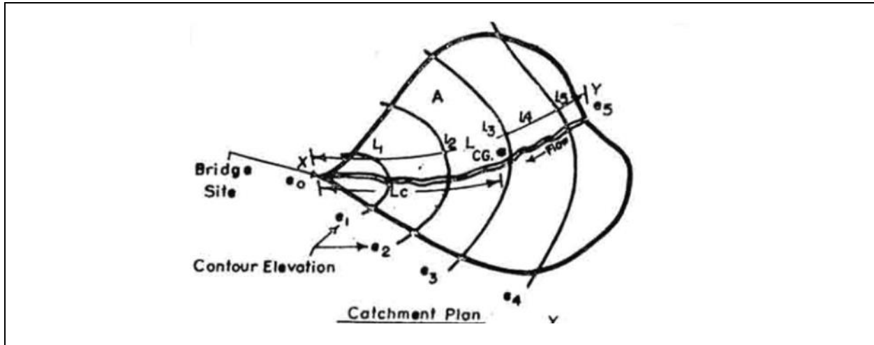
Fig.-4 Catchment plan for ungauged sites
