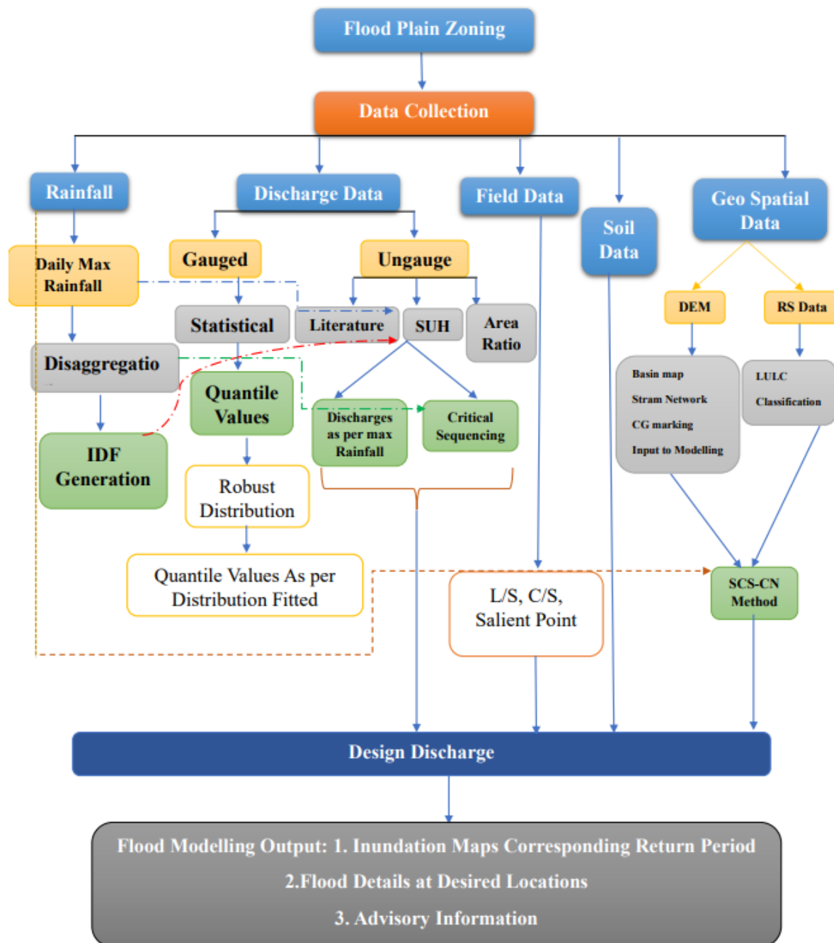
Fig.-6 Steps for Design Discharge calculations and subsequent modelling
