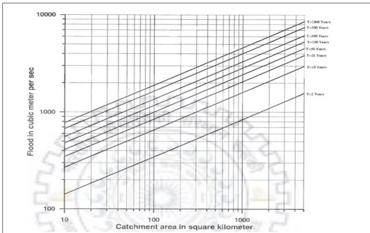
Fig. 17 Variation of floods of Various return periods with catchment area based on L-moments for Sub-Himalayan region Zone-7
