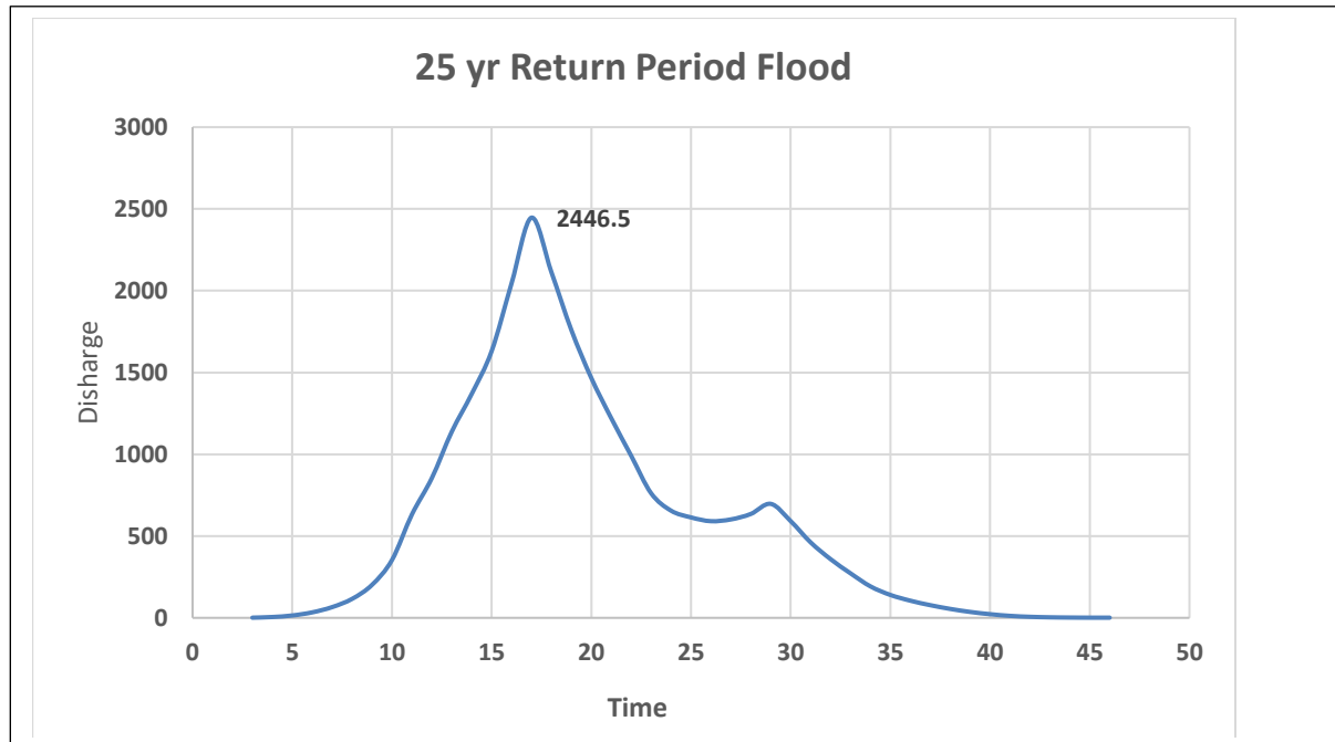
Fig. 13: Design Flood Hydrograph for 25yr Return Period
