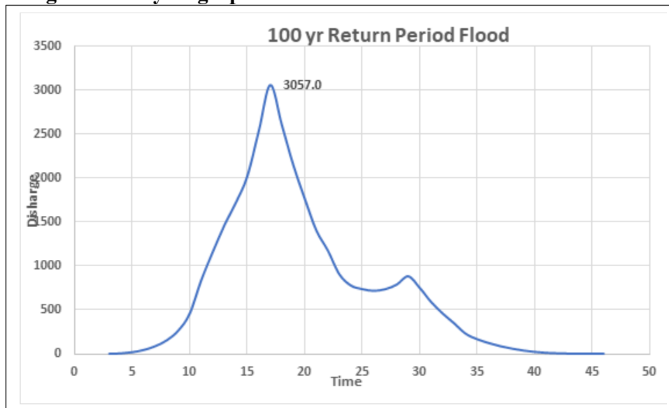
Fig.11: Design Flood Hydrograph for 100yr Return Period
