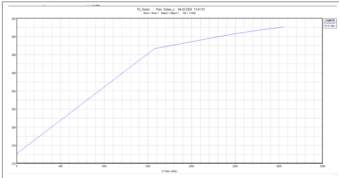
Fig. 22: Rating Curve of Solani River.
